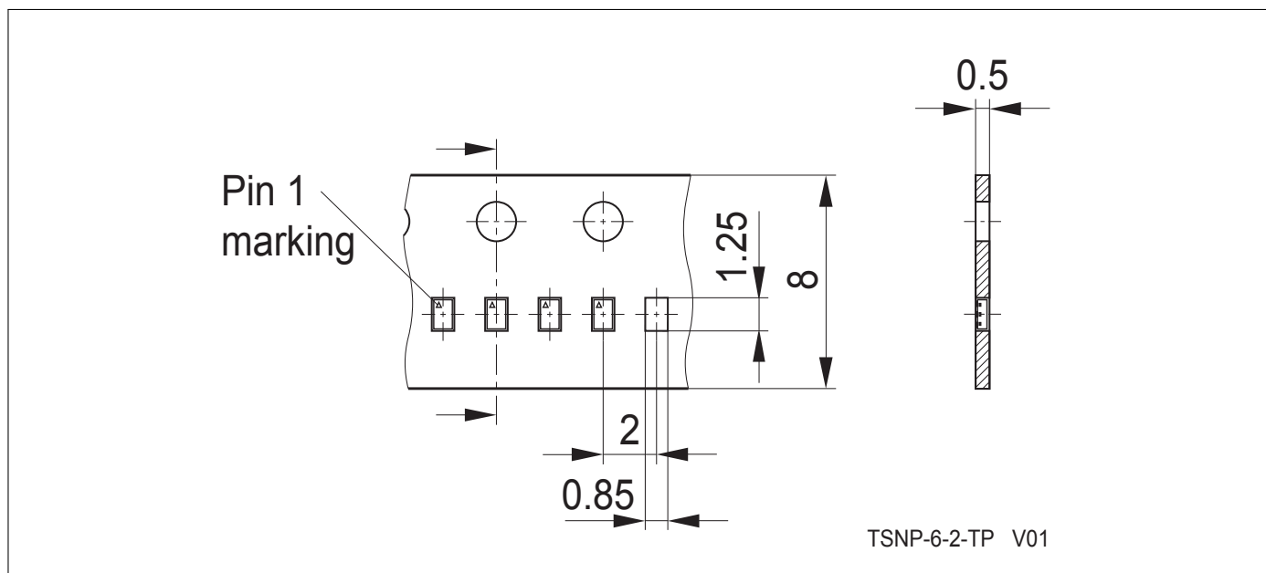
Figure 8: Tape Drawing (TSNP-6-2)
