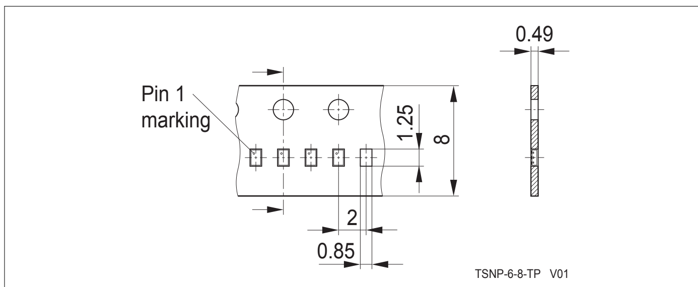
Figure 9: Tape Drawing (TSNP-6-8)
