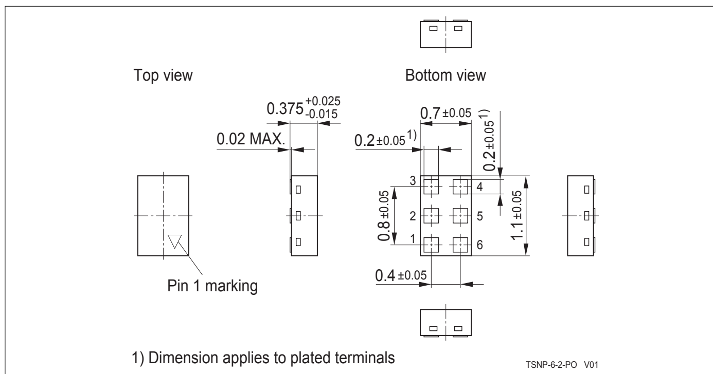
Figure 3: Package Outline (TSNP-6-2)
