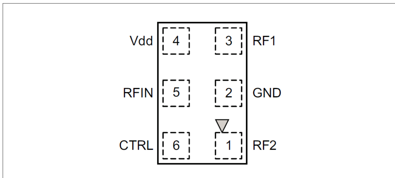
Figure 2: Pin Configuration
