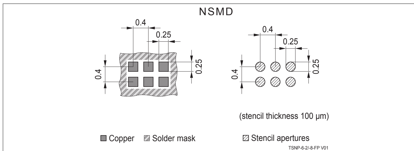
Figure 5: Footprint (TSNP-6-2/-8)
