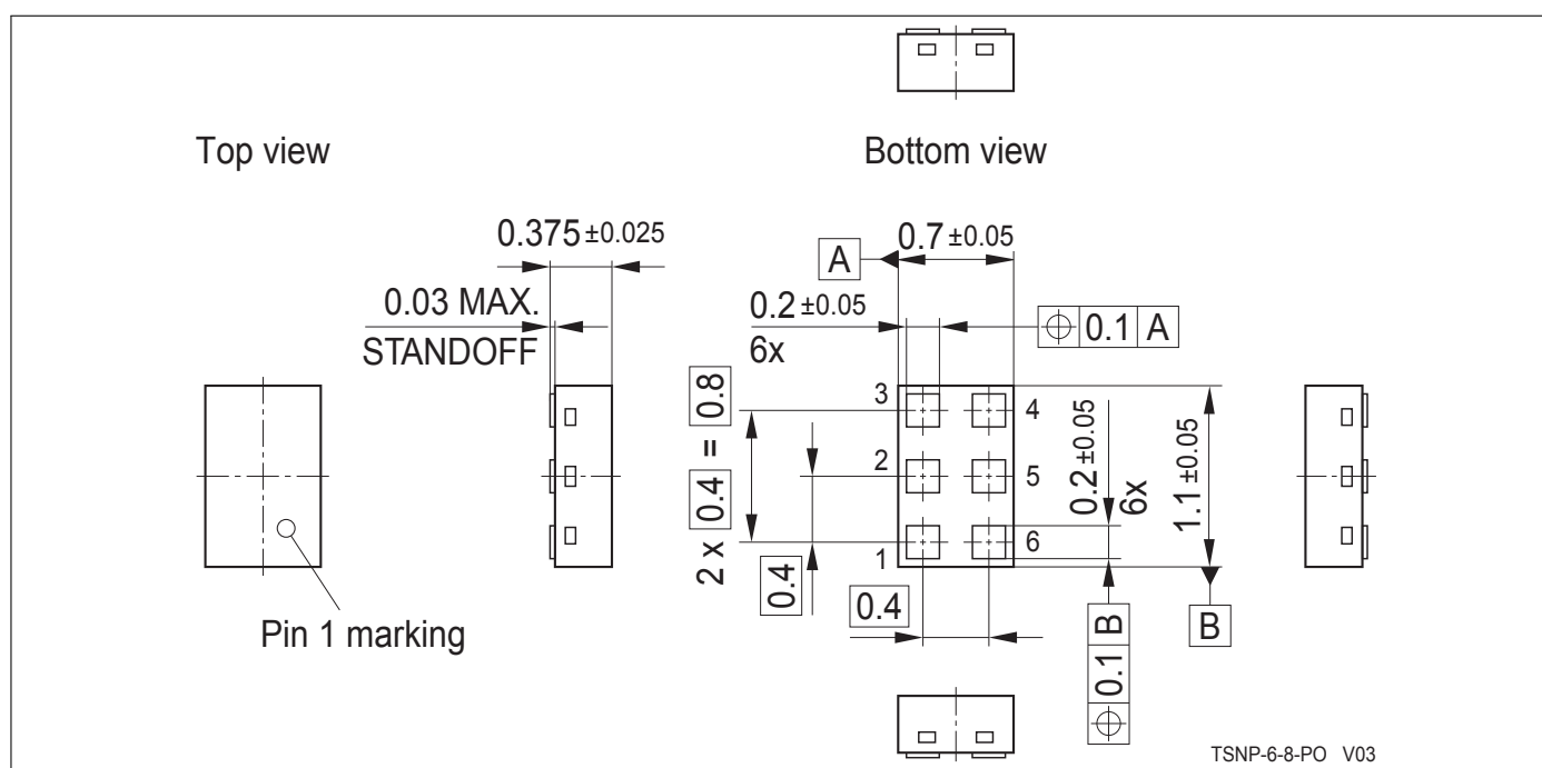
Figure 4: Package Outline (TSNP-6-8)
