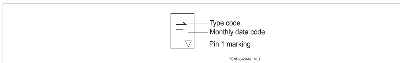
Figure 6: Pin 1 Marking (TSNP-6-2 top view)
