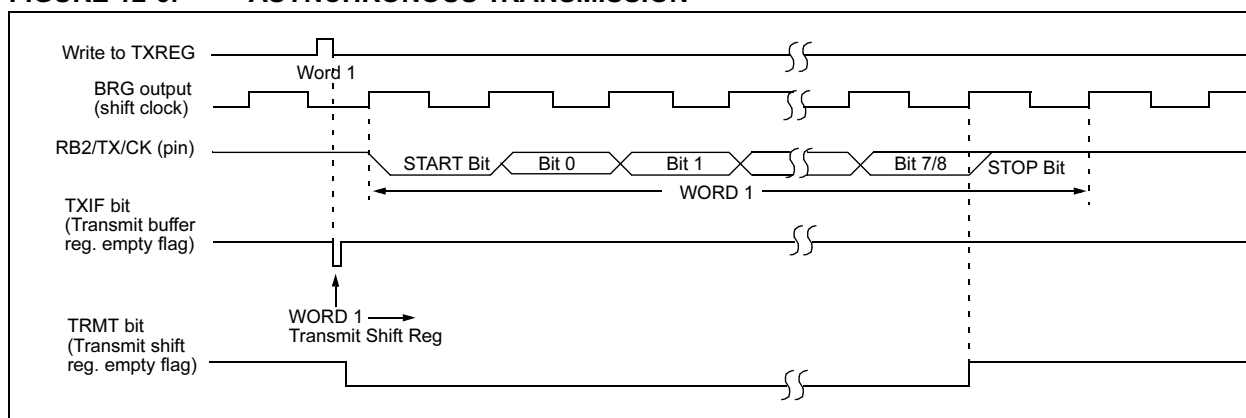
FIGURE 12-6: ASYNCHRONOUS TRANSMISSION
