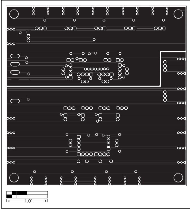
Figure 7. MAX9121 EV Kit PC Board Layout—Inner Layer 3
