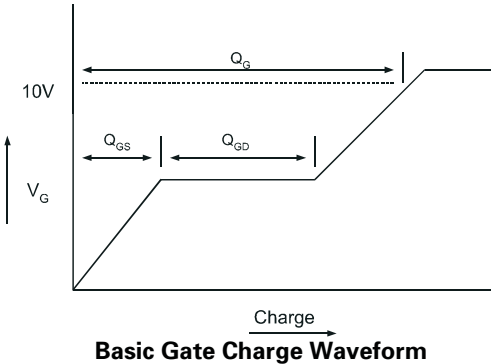
Basic Gate Charge Waveform
