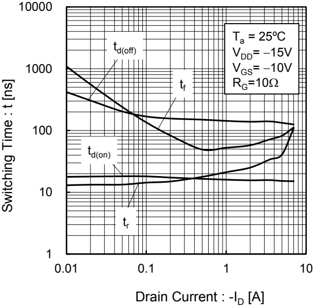
Fig.19 Switching Characteristics
