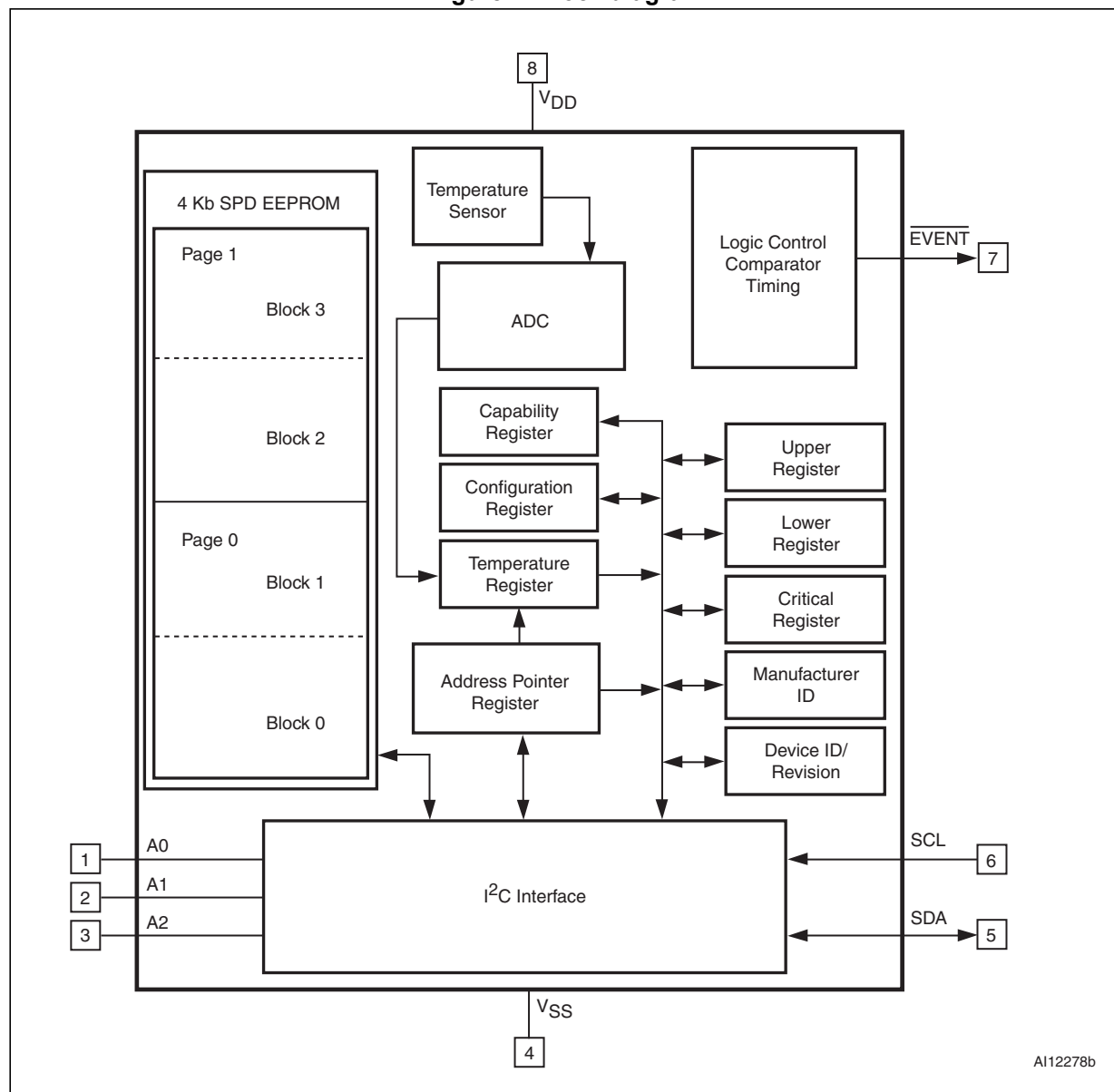
Figure 4. Block diagram
