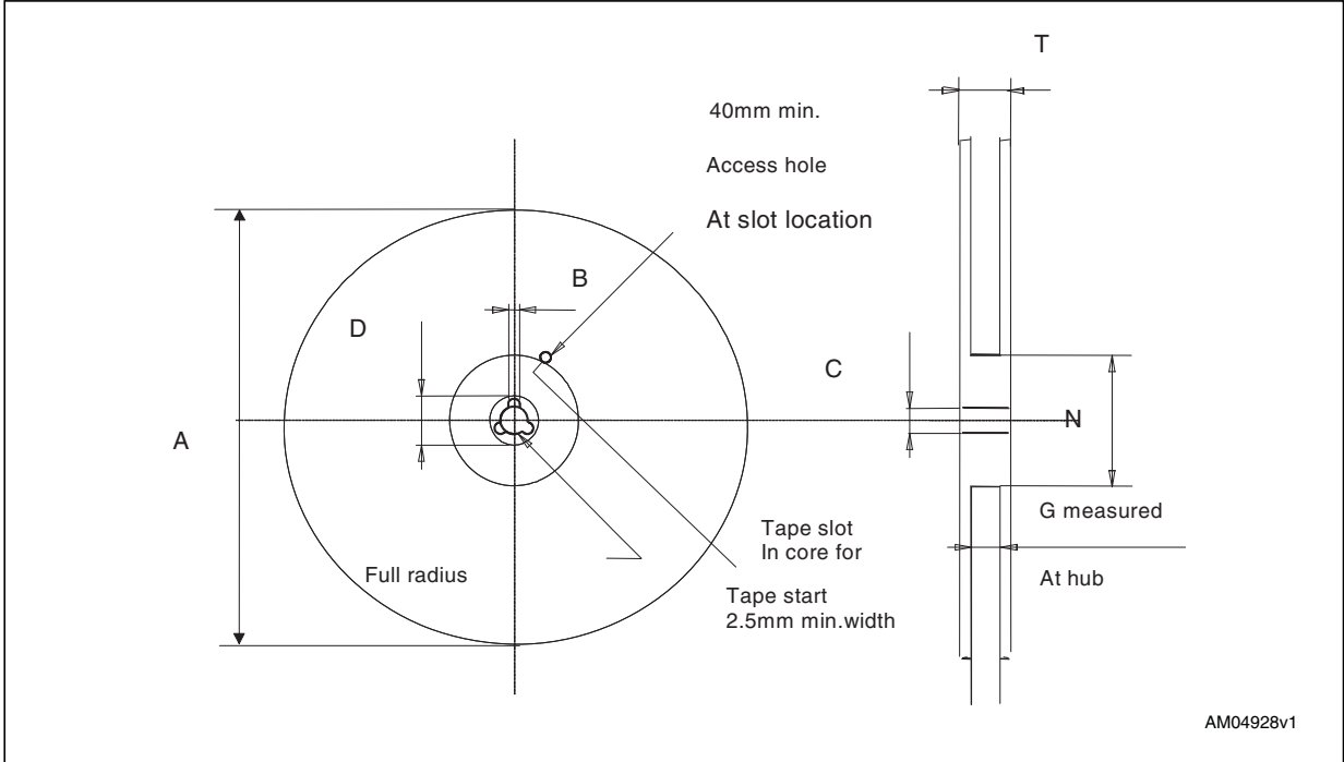
Figure 25. Reel schematic
