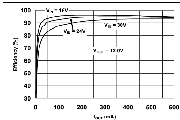
FIGURE 2-4: 12V V_{OUT} Efficiency vs. I_{OUT} .
