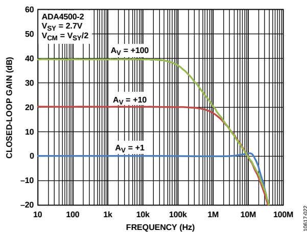
Figure 25. Closed Loop Gain vs. Frequency, V_{SY} = 2.7\text{ V}
