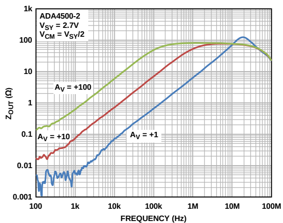
Figure 31. Closed Loop Output Impedance ( Z_{OUT} ) vs. Frequency, V_{SV} = 2.7\text{ V}
