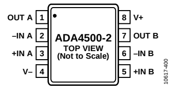
Figure 3. 8-Lead MSOP Pin Configuration
