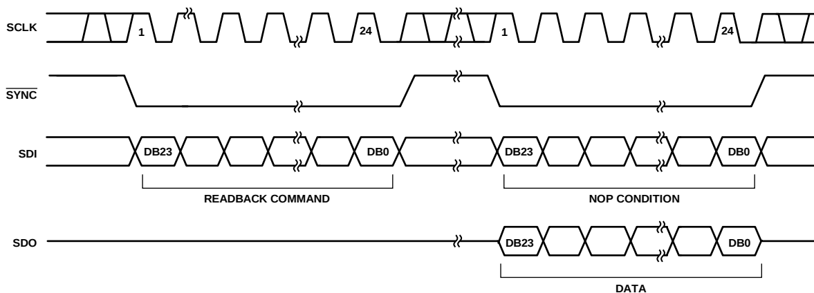
Figure 53. Readback Operation
