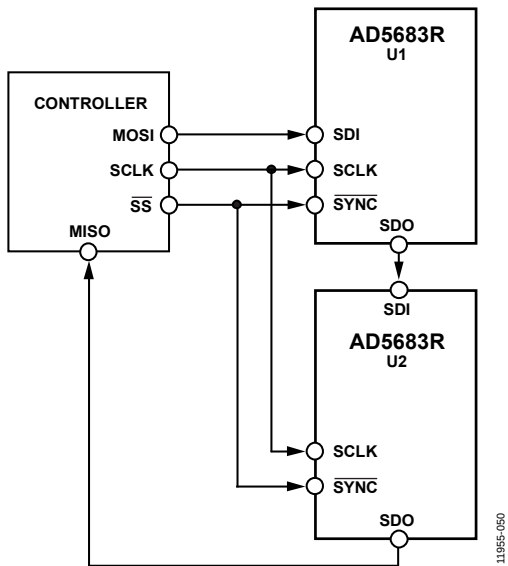
Figure 50. Daisy-Chain Connection
