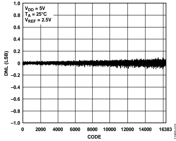
Figure 15. AD5682R DNL
