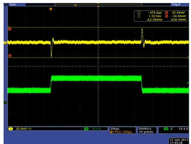
FIGURE 14. STEP RESPONSE, 10A TO 20A @ 5A/μs, ASCR = 400 TOTAL DEVIATION WINDOW 50mV = 5%
