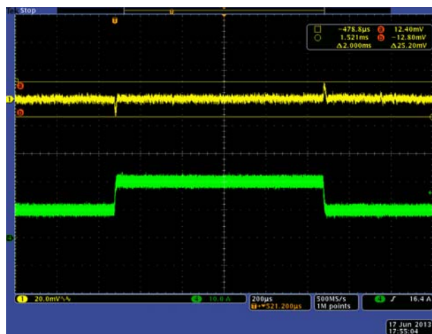
FIGURE 13. STEP RESPONSE, 10A TO 20A @ 5A/μs, ASCR = 1000 TOTAL DEVIATION WINDOW 25mV = 2.5%
