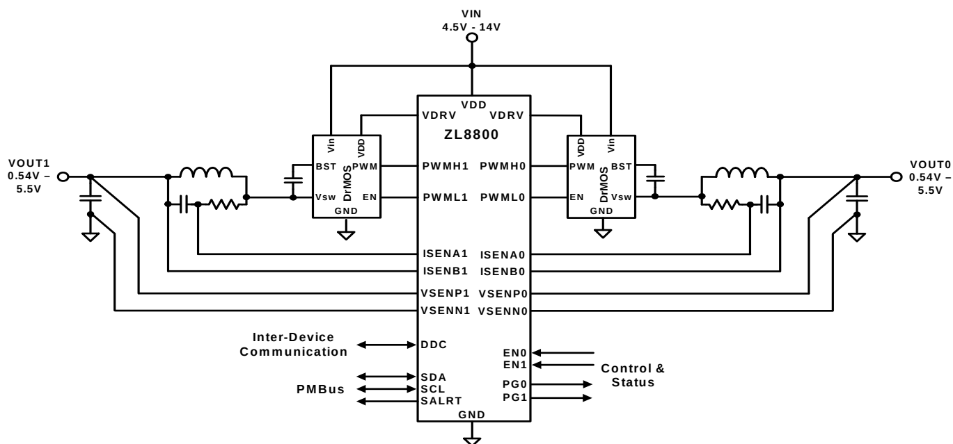
FIGURE 1. ZL8800-2CH-DEM01Z SIMPLIFIED SCHEMATIC
