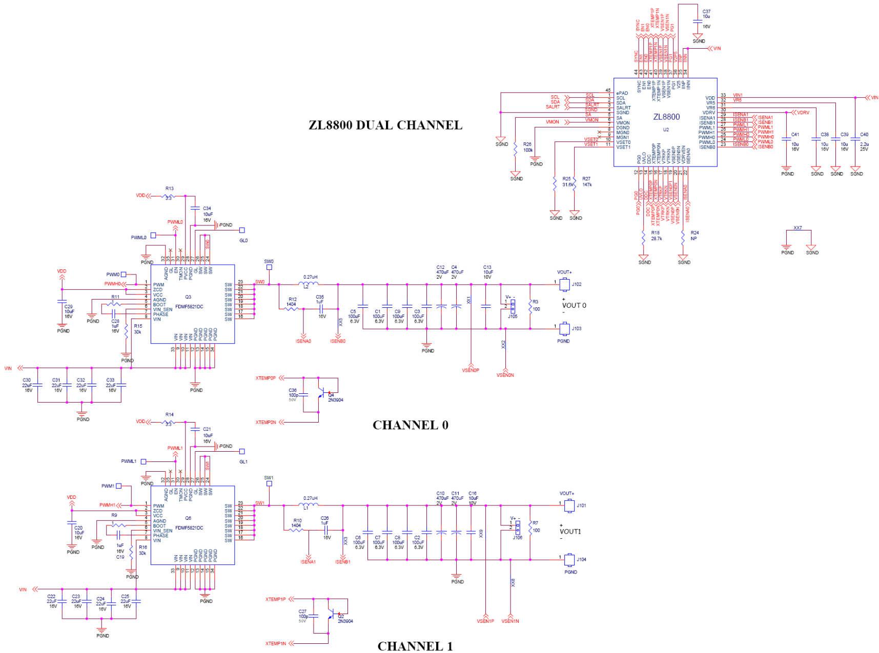
FIGURE 2. APPLICATION CIRCUIT
