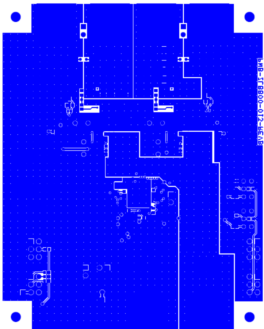
FIGURE 21. PCB - BOTTOM LAYER (TOP VIEW)
