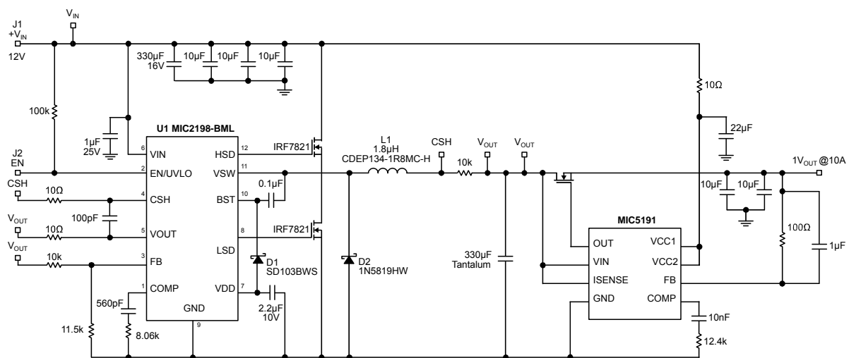
Figure 9. Post Regulator
