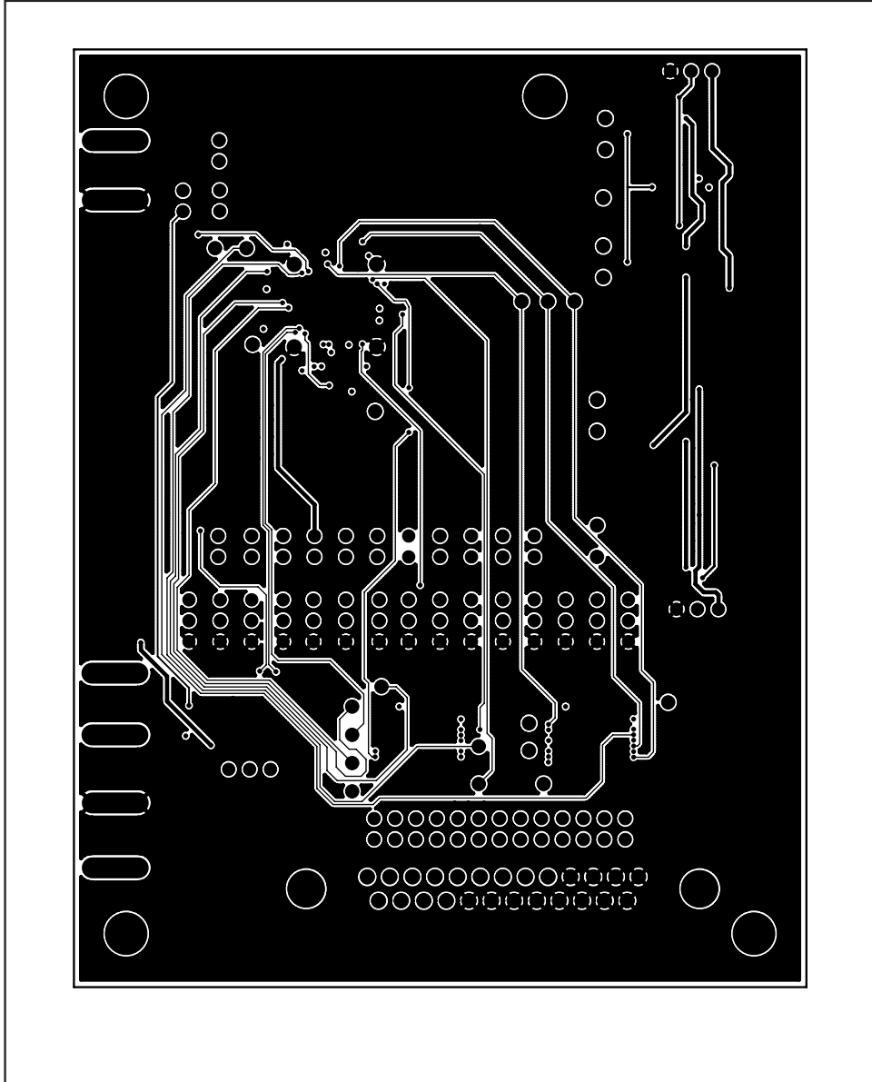
Figure 5. MAX2830 EV Kit PCB Layout—Inner Layer 3 (Routes)
