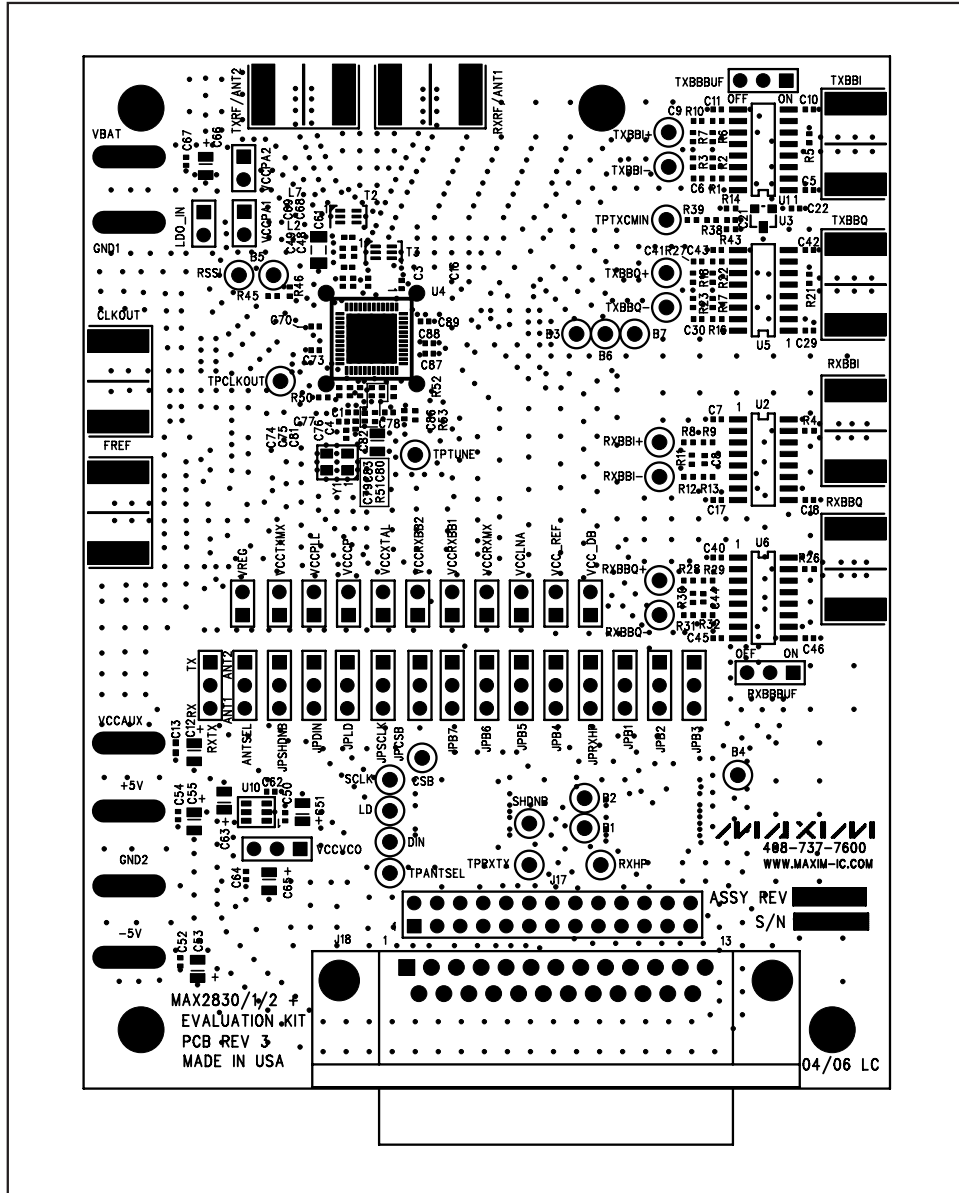
Figure 2. MAX2830 EV Kit PCB Layout—Top Silkscreen
