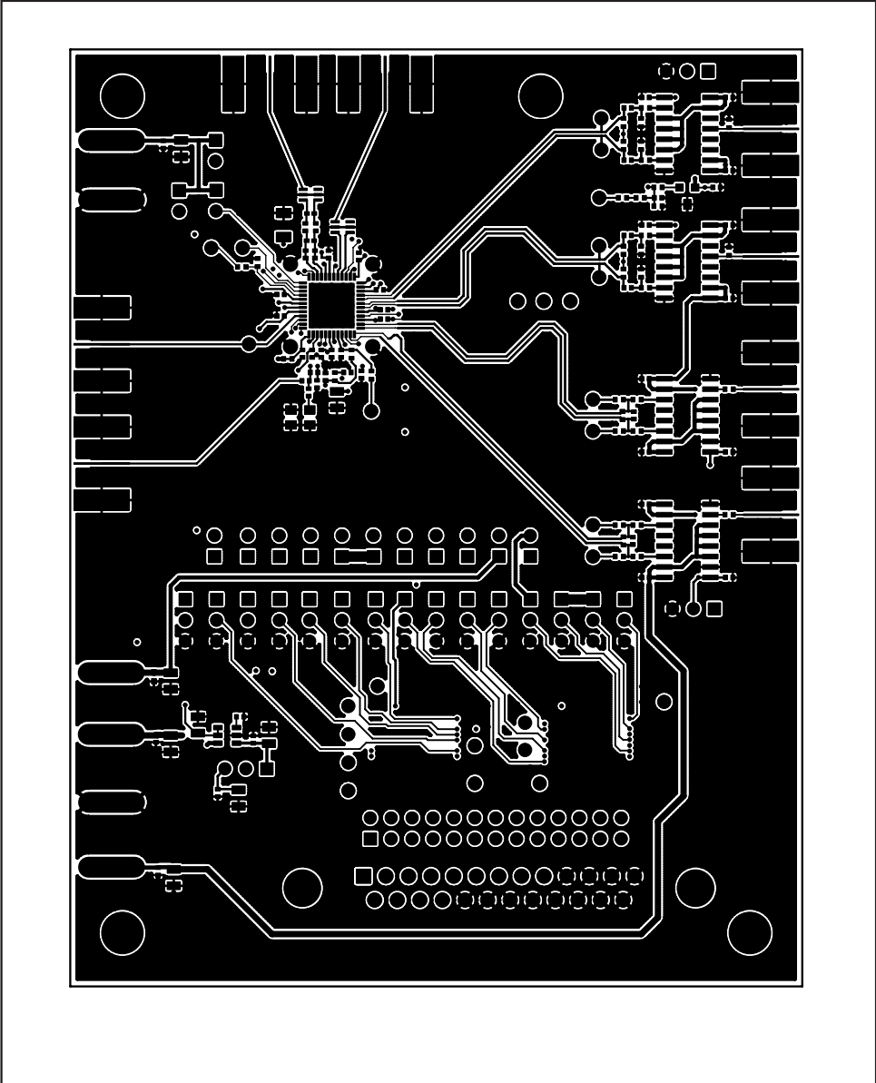
Figure 3. MAX2830 EV Kit PCB Layout—Component Side
