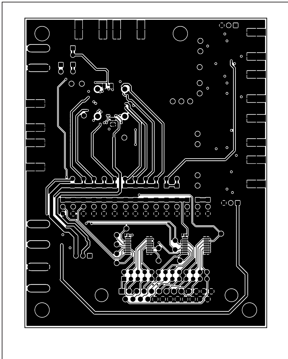
Figure 6. MAX2830 EV Kit PCB Layout—Solder Side
