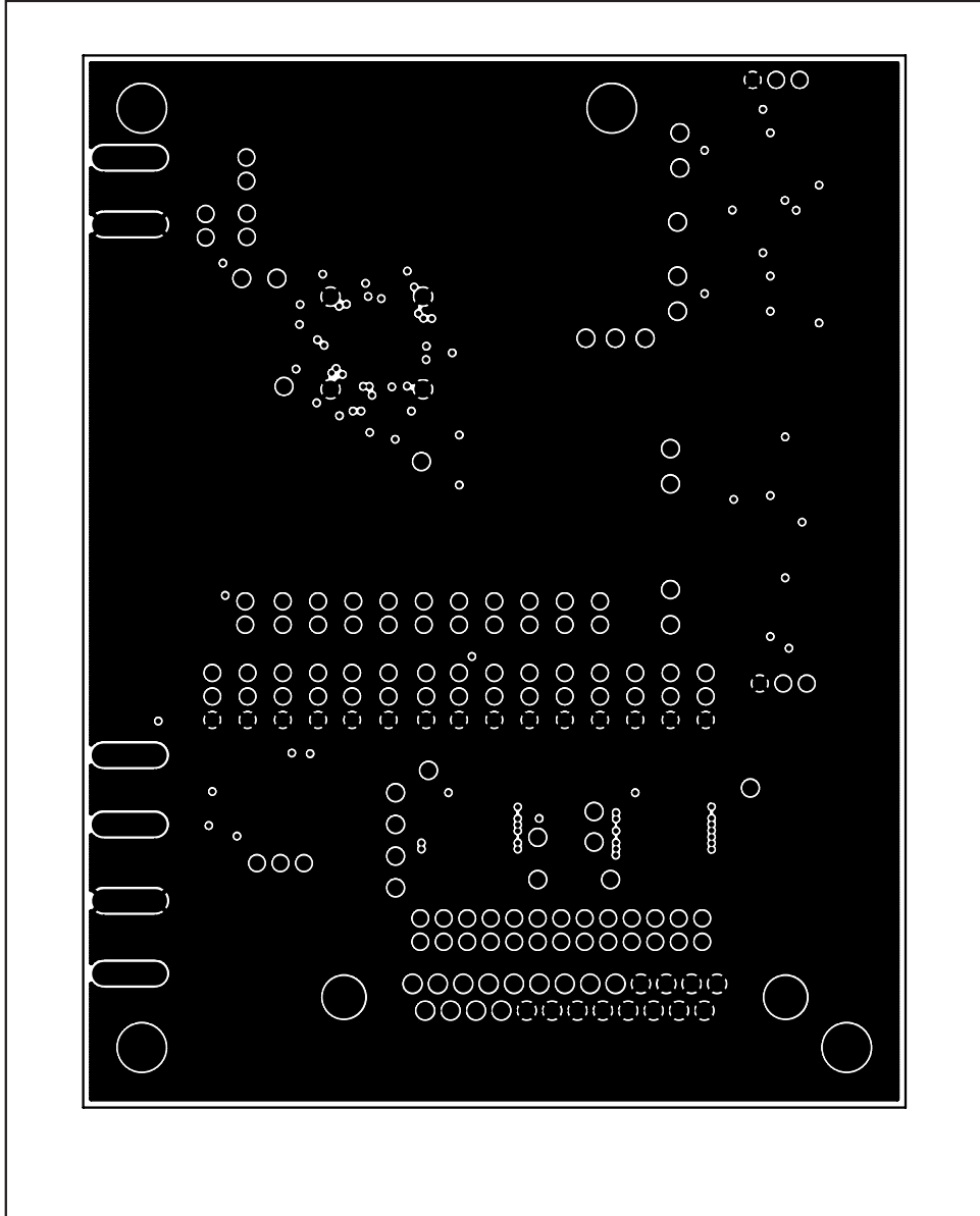
Figure 4. MAX2830 EV Kit PCB Layout—Inner Layer 2 (Ground Layer)
