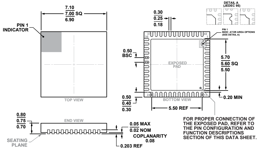
Figure 77. 48-Lead Lead Frame Chip Scale Package [LFCS] 7 mm × 7 mm Body and 0.75 mm Package Height (CP-48-13) Dimensions shown in millimeters
