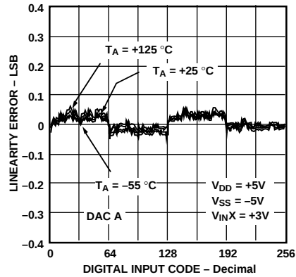
Figure 5. Linearity Error vs. Digital Code vs. Temperature
