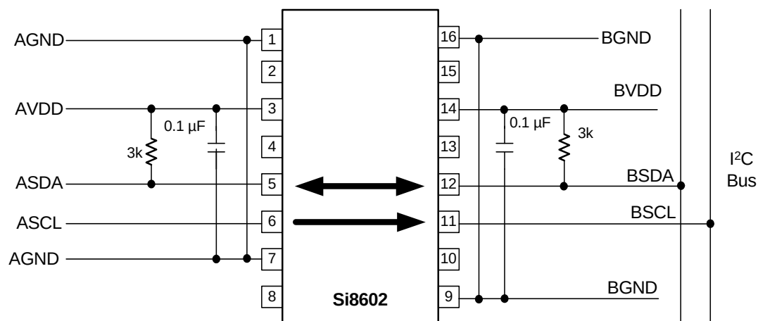
Figure 13. Typical Si8602 Application Diagram
