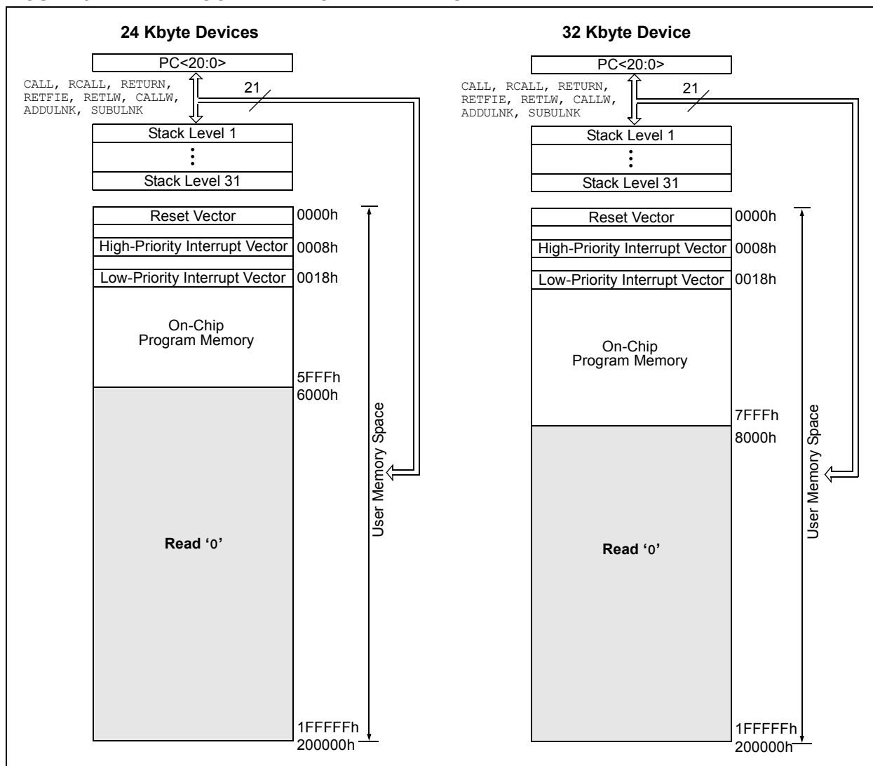
FIGURE 5-1: PROGRAM MEMORY MAP AND STACK
