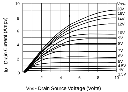
Saturation Characteristics
