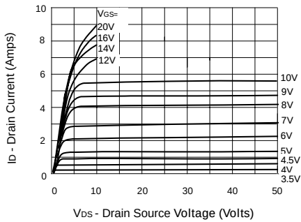
Output Characteristics
