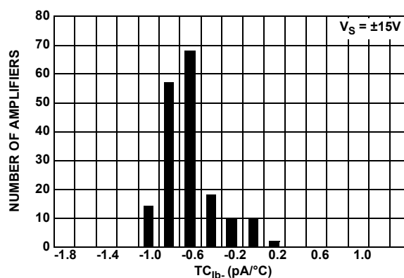
FIGURE 16. TC_{1b-} vs NUMBER OF AMPLIFIERS, V_S = \pm 15V
