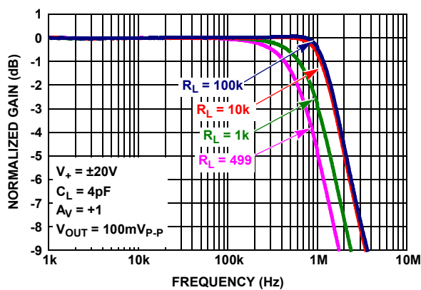
FIGURE 44. GAIN vs FREQUENCY vs R_L
