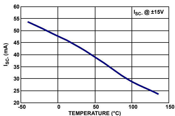
FIGURE 32. NEGATIVE SHORT CIRCUIT CURRENT vs TEMPERATURE
