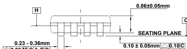
SIDE VIEW 1
