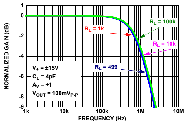
FIGURE 63. SIMULATED CLOSED LOOP GAIN vs R_L
