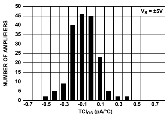
FIGURE 20. TC_{IOS-} vs NUMBER OF AMPLIFIERS, V_S = \pm 5V
