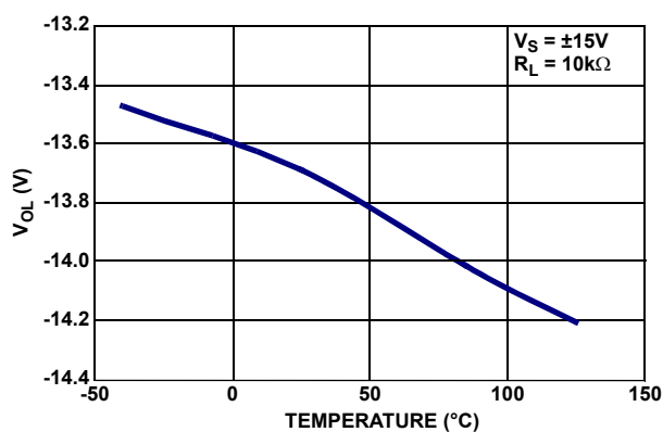
FIGURE 25. V_{OL} vs TEMPERATURE, V_S = \pm 15V , R_L = 10k\Omega
