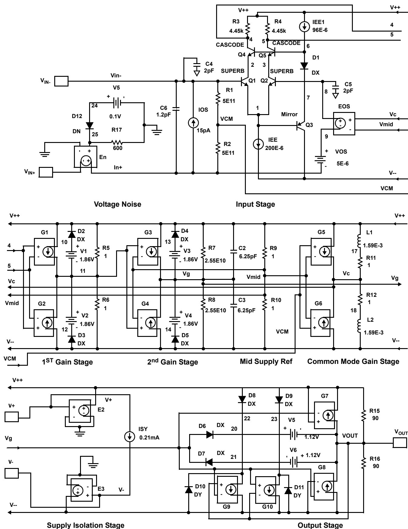
FIGURE 56. SPICE SCHEMATIC
