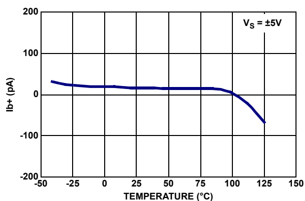
FIGURE 10. POSITIVE BIAS CURRENT vs TEMPERATURE, V_S = \pm 5V
