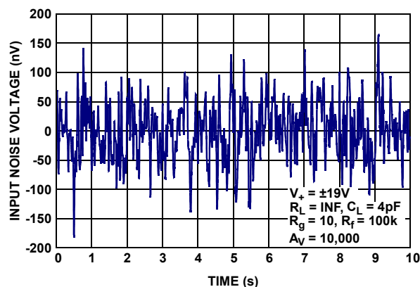
FIGURE 33. INPUT NOISE VOLTAGE 0.1Hz TO 10Hz
