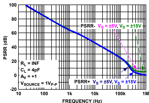
FIGURE 36. PSRR vs FREQUENCY, V_S = \pm 5V , \pm 15V
