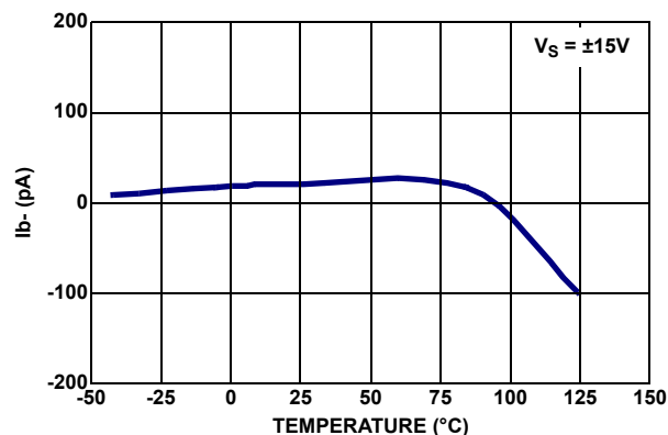
FIGURE 13. NEGATIVE BIAS CURRENT vs TEMPERATURE, V_S = \pm 15V
