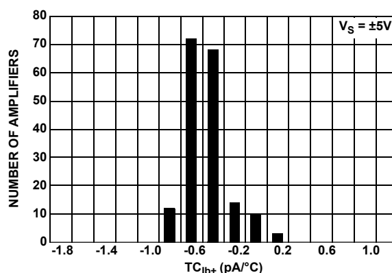
FIGURE 12. TC_{Ib+} vs NUMBER OF AMPLIFIERS, V_S = \pm 5V
