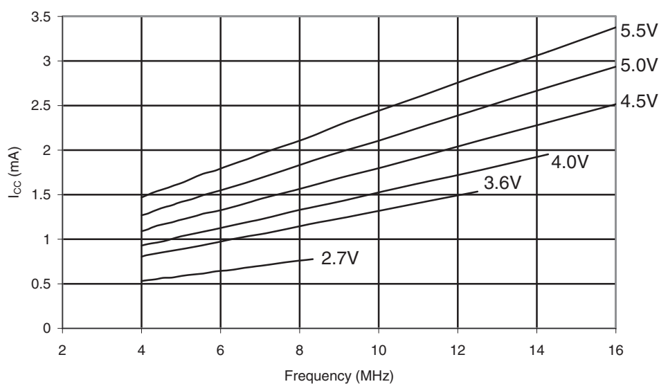
Figure 30-43. Reset Supply Current vs. Frequency (1 - 20MHz)
