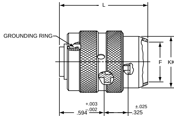
LJT06RP-XX-XXX (MS27467P)
