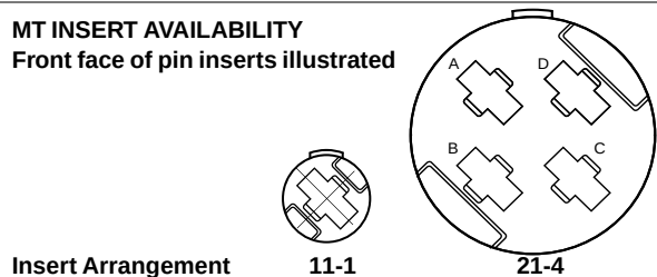
MT38999 Connectors
