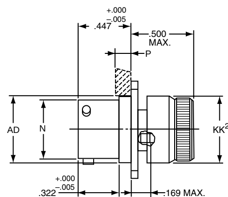
* JTPQ00RE-XX-XXX (MS27497E)
