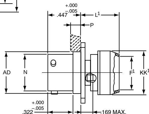
* JTPQ00RP-XX-XXX(MS27497P)
