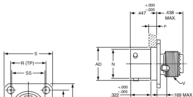
* JTPQ00RT-XX-XXX(MS27497T) ** JTPSQ00RT-XX-XXX
