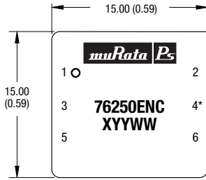
Pin Connections 76250EN (Top View)
