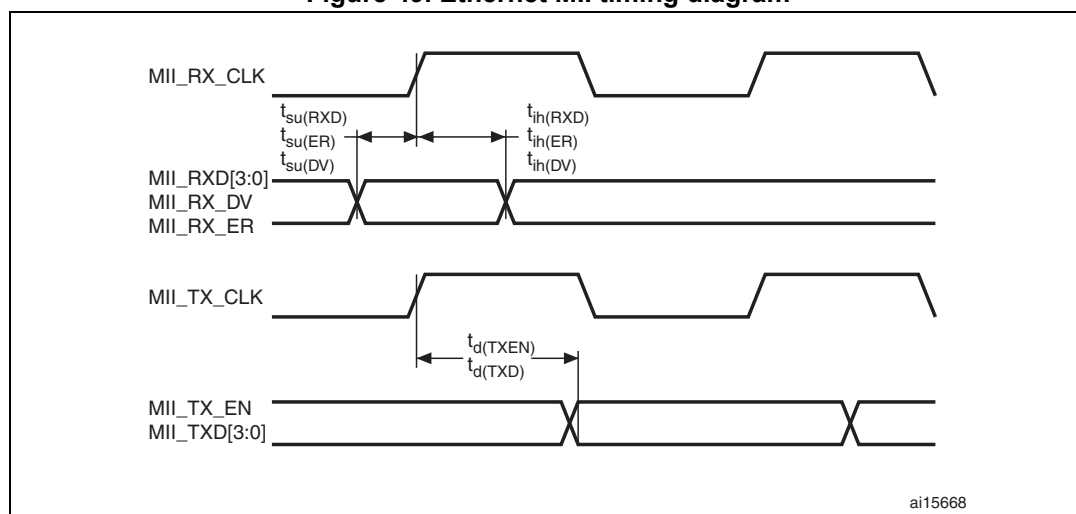
Figure 49. Ethernet MII timing diagram
