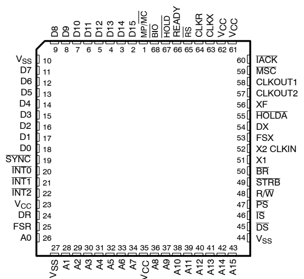
68-Pin FN and FZ Packages† (Top View)
