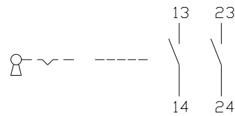
15 Keylock switch 2 positions page 8
