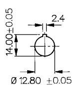
Fixing Details
