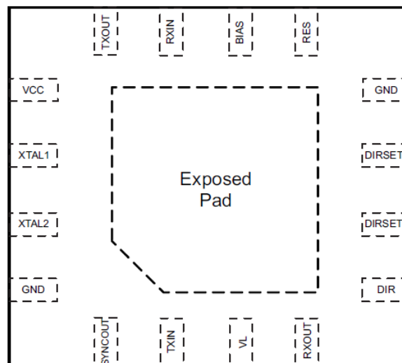
Figure 1. SN65HVD62 Pinout
