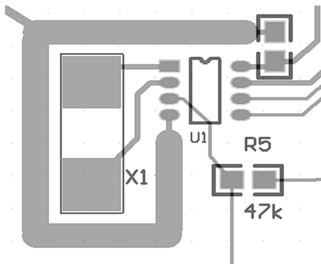
FIGURE 23. SUGGESTED LAYOUT FOR INTERSIL RTC IN 8 Ld SOIC PACKAGE
