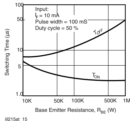
Fig. 15 - Typical Switching Characteristics vs. Base Resistance (Saturated Operation)
