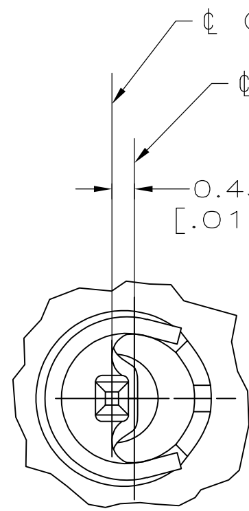
VIEW B-B SCALE 10:1 5 PLC
