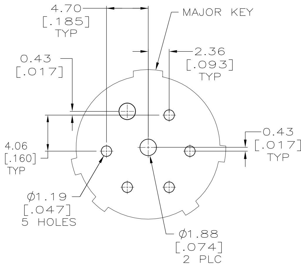
RECOMMENDED BOARD LAYOUT FOR 788194-1, -3 & -5 SCALE 4:1
