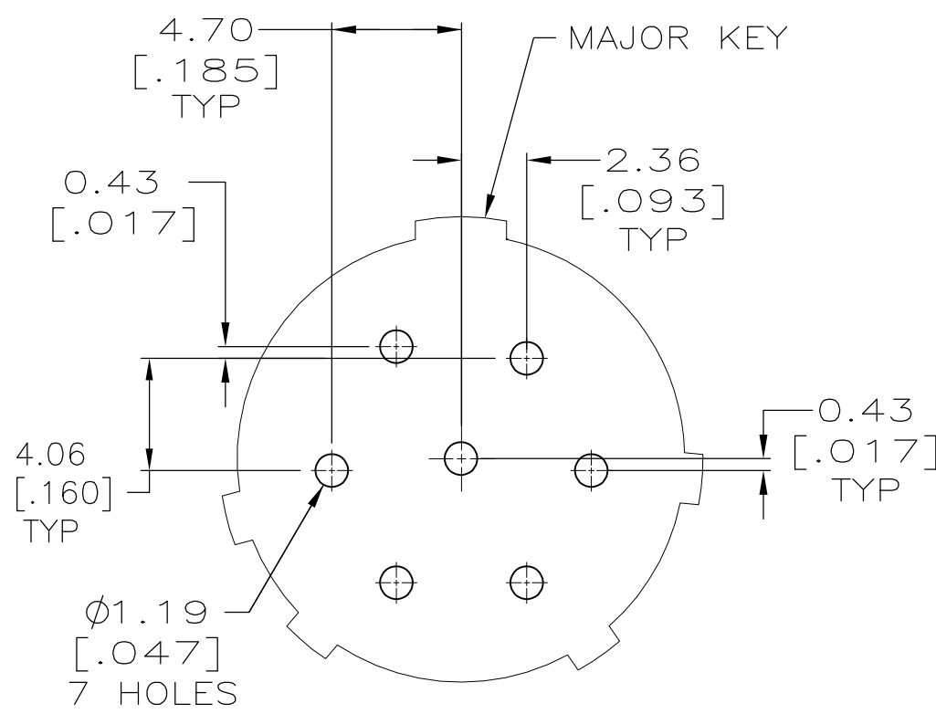
RECOMMENDED BOARD LAYOUT FOR 788194-2 & -4 SCALE 4:1
