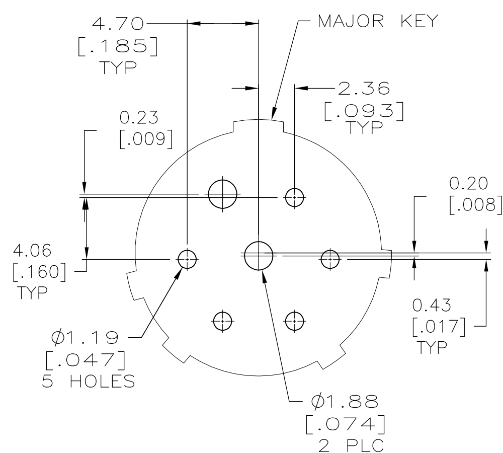
RECOMMENDED BOARD LAYOUT FOR 788194-6 ONLY SCALE 4:1
