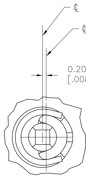
VIEW C-C SCALE 10:1 2 PLC 788194-6 ONLY
