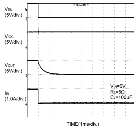
Fig.30 Output fall characteristic
