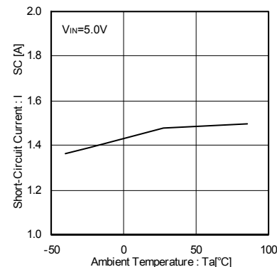
Fig.14 Short circuit current
