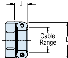
STYLE A Medium Duty (Table V)
