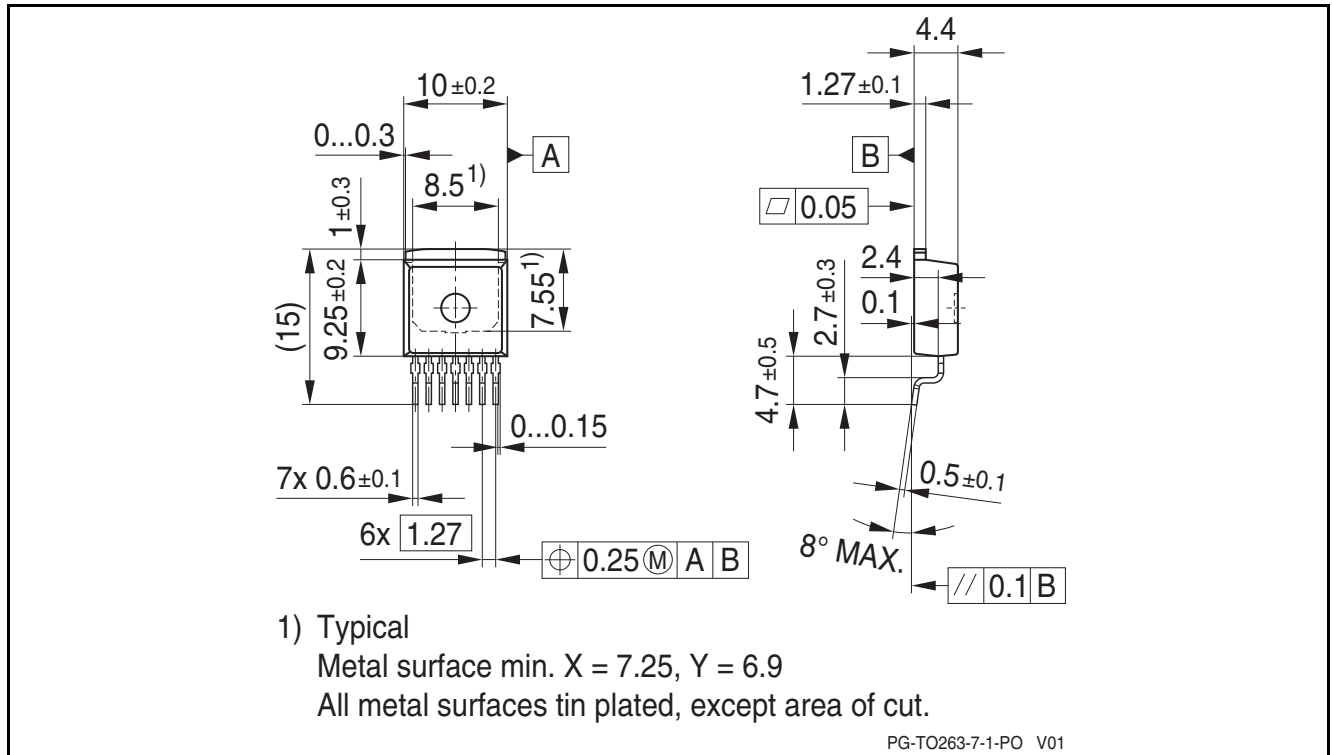
Figure 1 PG-T0263-7-1
