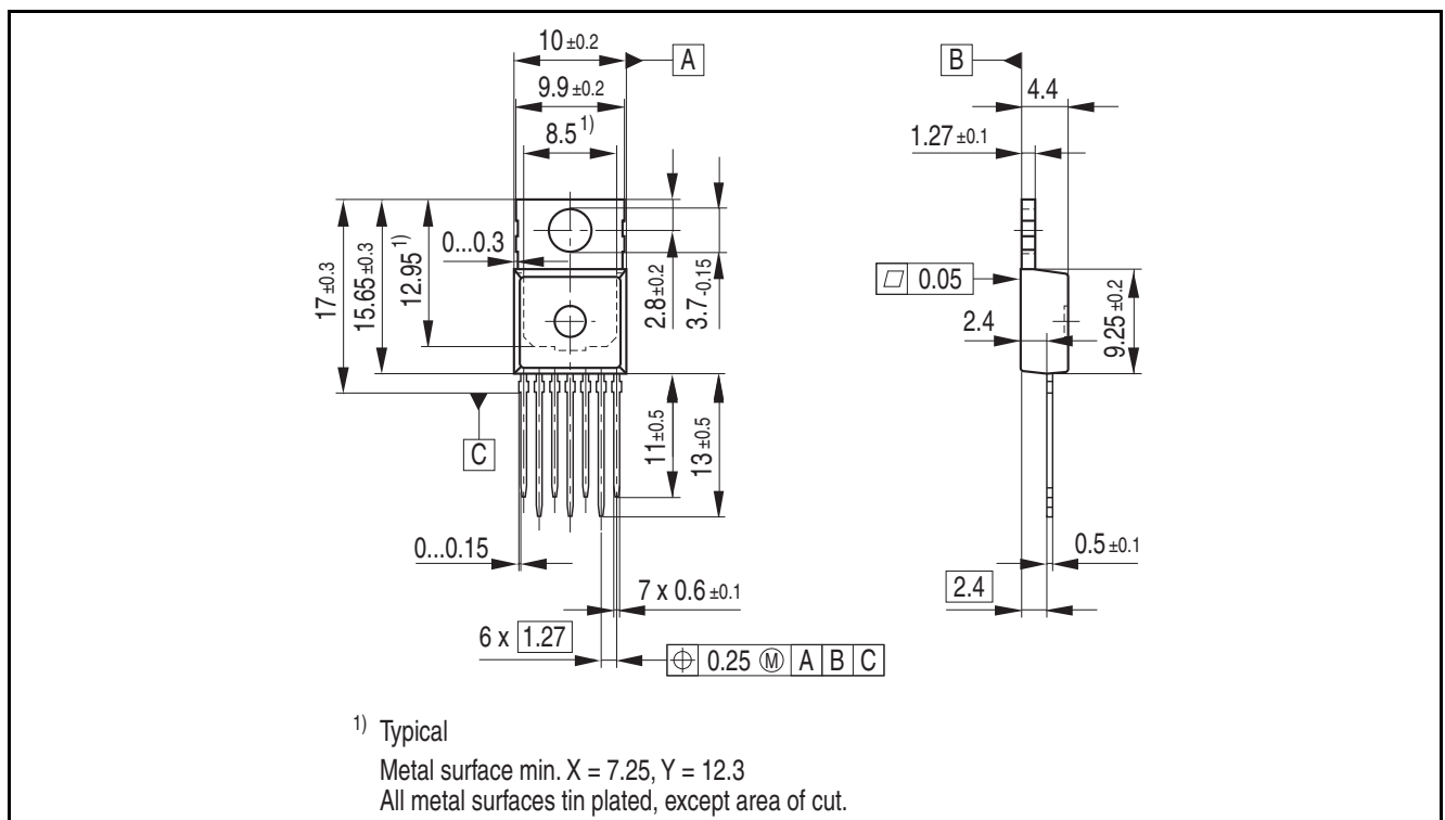
Figure 2 PG-T0220-7-12
