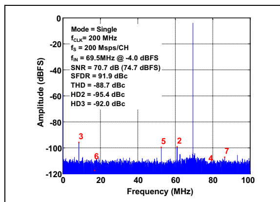
FIGURE 3-5: FFT for 69.5 MHz Input Signal: f_S = 200\text{ Mps/Ch.} , A_{IN} = -4\text{ dBFS} .
