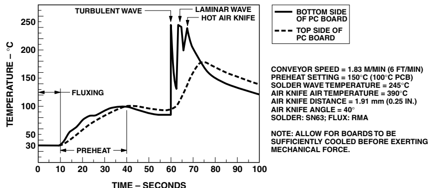
Figure 7. Recommended wave soldering profile.
