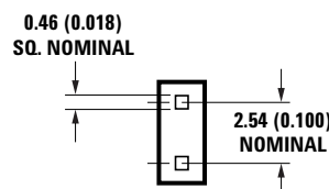
BOTTOM VIEW
