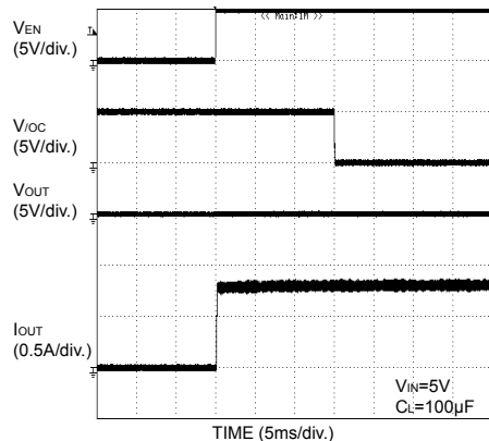
Fig.34 Over-current response enable to shortcircuit
