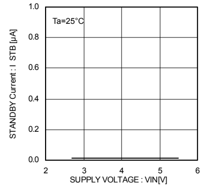
Fig.5 Standby current EN, /EN disable
