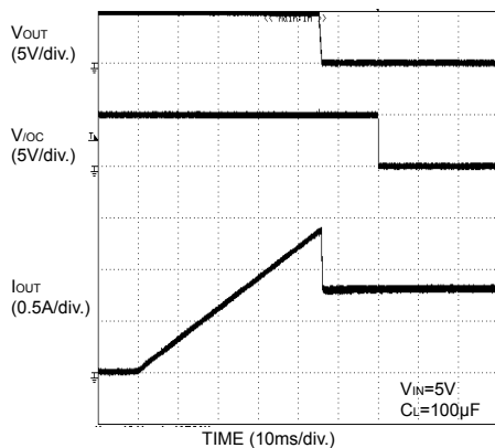
Fig.32 Over-current response ramped load
