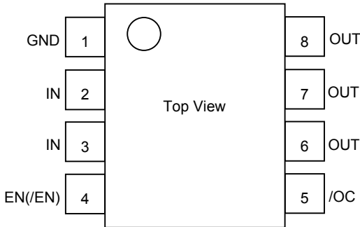
Fig.40 Pin configuration
