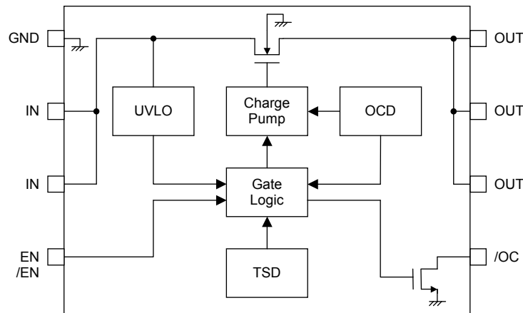
Fig.39 Block diagram
