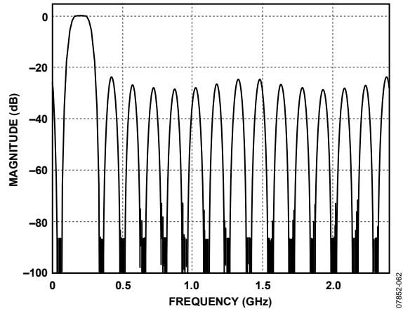
Figure 89. Band-Pass Filter Response at 200 MHz, f_{DAC} = 2.4 GHz
