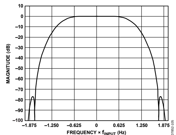
Figure 82. 2\times Half-Band Interpolation Filter 3 and Filter 4 Response
