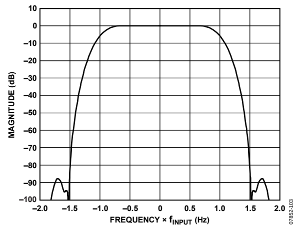
Figure 80. 2\times Half-Band Interpolation Filter 1 Response
