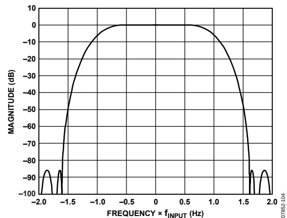
Figure 81. 2\times Half-Band Interpolation Filter 2 Response
