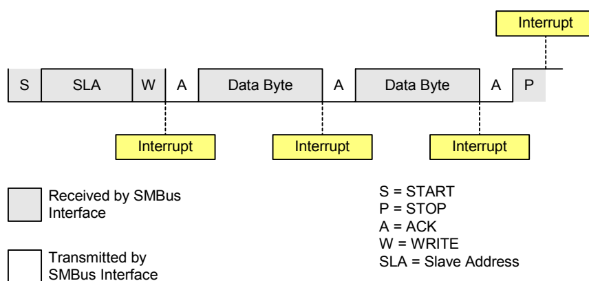
Figure 18.7. Typical Slave Receiver Sequence
