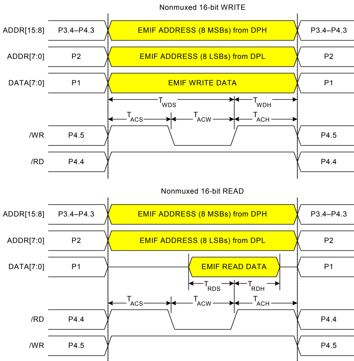
Figure 15.4. Non-multiplexed 16-bit MOVX Timing
