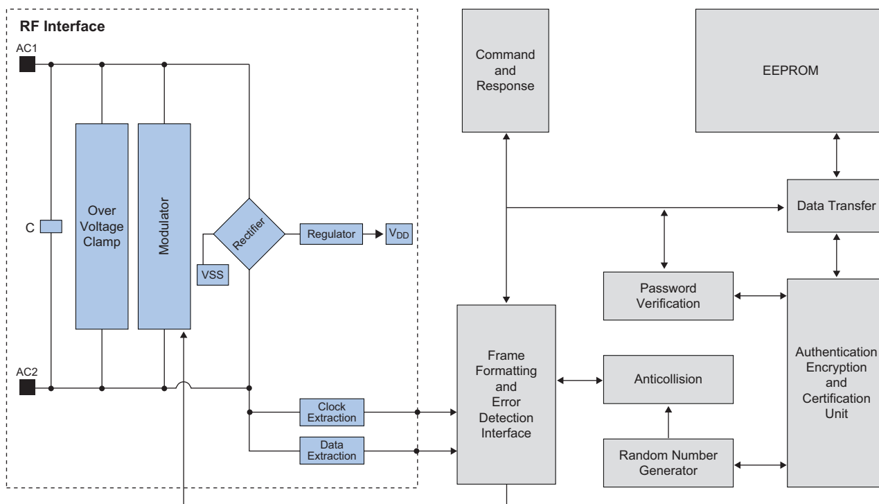
Figure 2-1. Block Diagram
