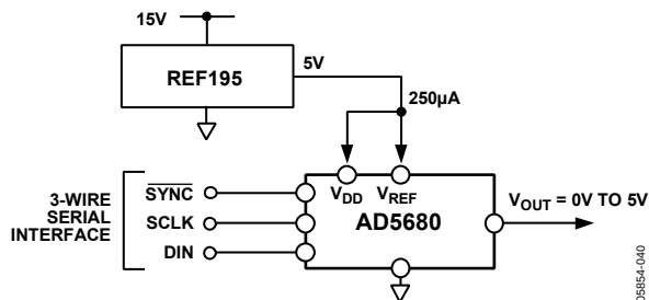
Figure 35. REF195 as Power Supply to the AD5680
