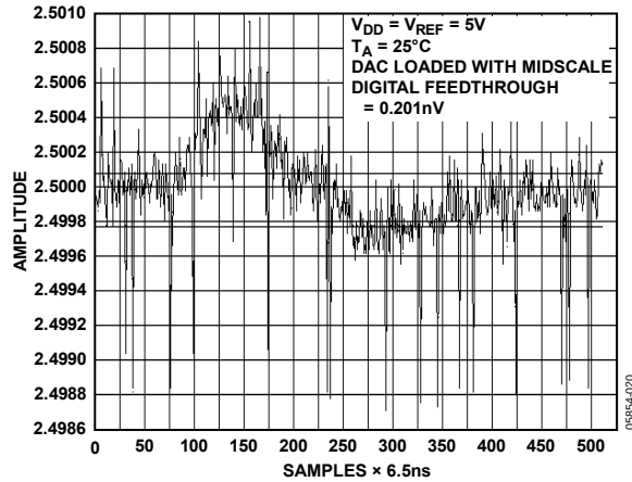
Figure 17. Digital Feedthrough
