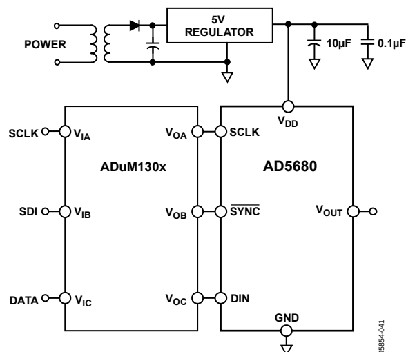
Figure 36. AD5680 with a Galvanically Isolated Interface
