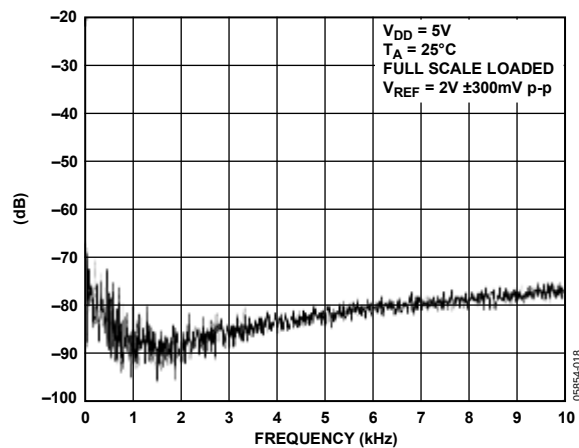
Figure 18. Total Harmonic Distortion
