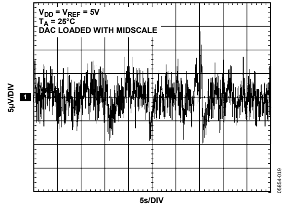
Figure 20. 0.1 Hz to 10 Hz Output Noise Plot
